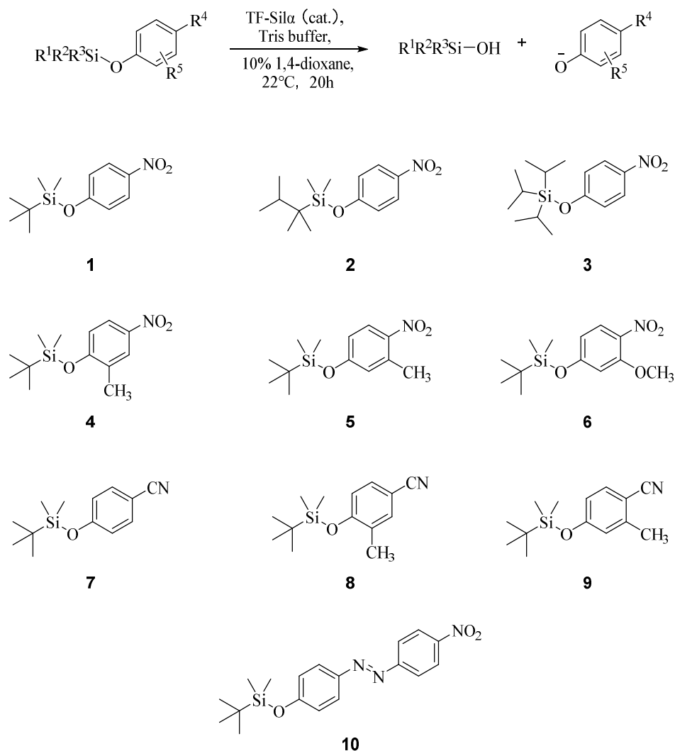
Scheme 1. Biocatalytic hydrolysis of phenoxy silyl ethers, with the structures of the various substrates shown below. R n = various substituents as shown in the individual structures.
