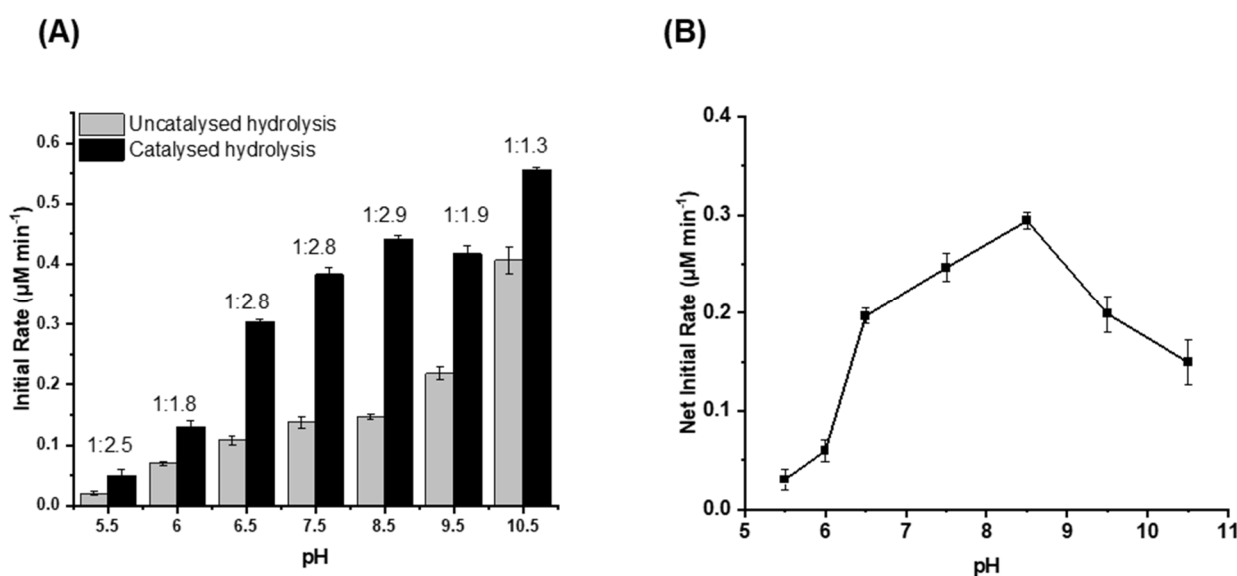
Figure 1. Plots of initial rate of hydrolysis of 1 against pH for (A) reactions that are uncatalysed (enzyme omitted) and catalysed (where the enzyme was present) and (B) the net enzymatic rate of hydrolysis. The net rate is calculated by subtracting the rate of the uncatalysed reaction from the reactions where the enzyme is present. The ratios of the catalysed to uncatalysed reactions are provided above each column pair. The error bars represent the standard error from triplicate experiments. Enzymatic reactions are carried out with 6.7 µM TF-Sil \alpha -Strep, 50 µM 1 , 10% v/v 1,4-dioxane, 50 mM Tris buffer at the appropriate pH and 100 mM NaCl.
