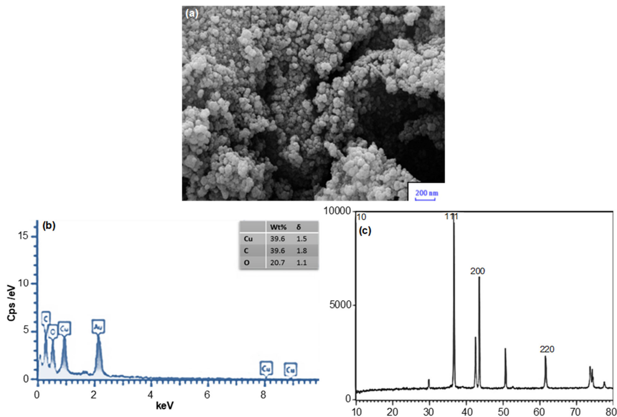
Fig 2. (a) SEM, (b) EDX, and (c) XRD analysis of CuNPs
