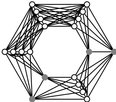
Figure 4. Construction for a = 4 and b = 6 : the lower mp-set.
