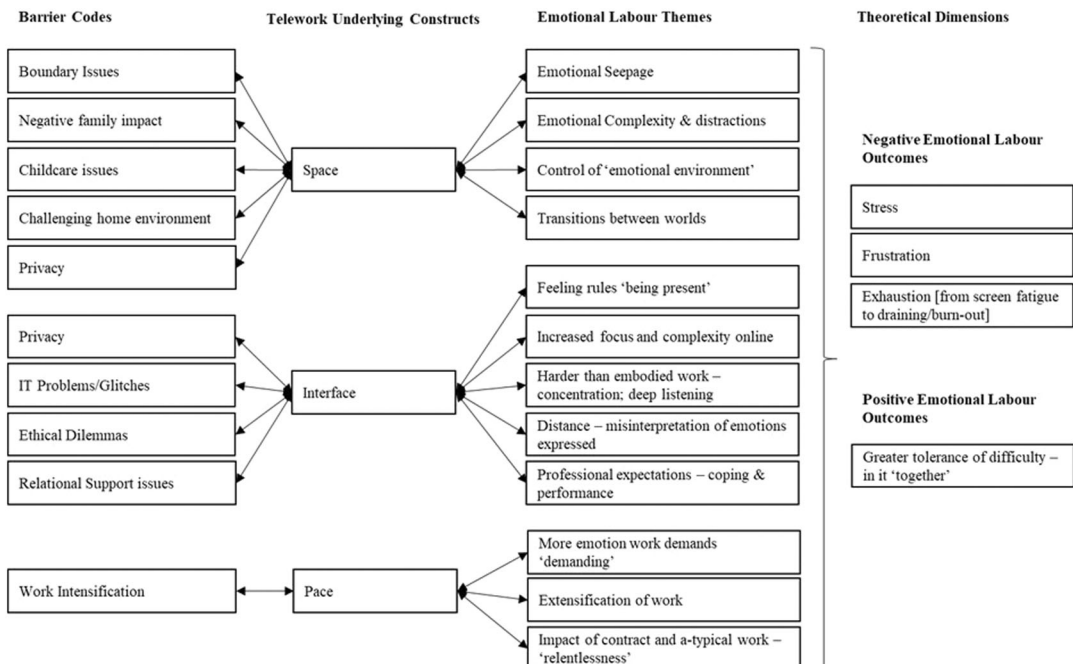
FIGURE 1 Data structure.
