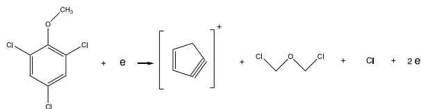
Reaction b. Dissociation leading to m/Z 62, with two neutral counterparts.
