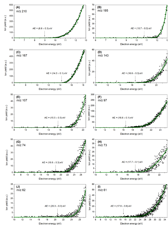
Fig. 2. Experimental thresholds for the ten most abundant cations (A)-(I), decreasing in m/z . The black dots represent the experimental data, and the green line represents the Wannier-type fitting function. The values in parentheses correspond to the experimental thresholds with the respective statistical uncertainties. Wannier-type fitting parameters are summarized in Table S2 (ESI).
