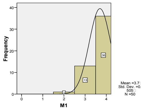
Figure 1-2 Histogram showing that marks are non-normally distributed
