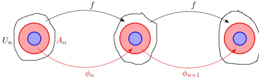
FIGURE 1. In the blue inner discs bounded by C_n , the original map f was replaced by appropriately translated versions of \gamma_n . To connect this with f , we interpolate on the red outer annuli A_n using the quasiconformal maps \phi_n .
