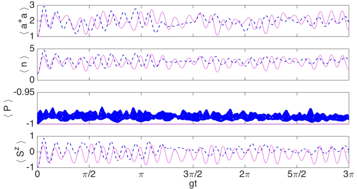
FIG. 10. Simulation of the anisotropic Dicke model in a two trapped-ion system in the DSC regime with parameters \nu = 2\pi \times 3\text{MHz} , \omega^0 = 2\pi \times 10^{14}\text{Hz} , \eta = 0.05 , \Gamma = \Omega\eta/100 , \Omega^r = 2\pi \times 50\text{kHz} , s = 5 , \delta^r = -2\pi \times 187\text{Hz} and \delta^b = -2\pi \times 12063\text{Hz} . Initial state: |1, \downarrow, \downarrow\rangle . Dotted magenta lines: anisotropic Dicke model, dashed blue lines: ion system.
