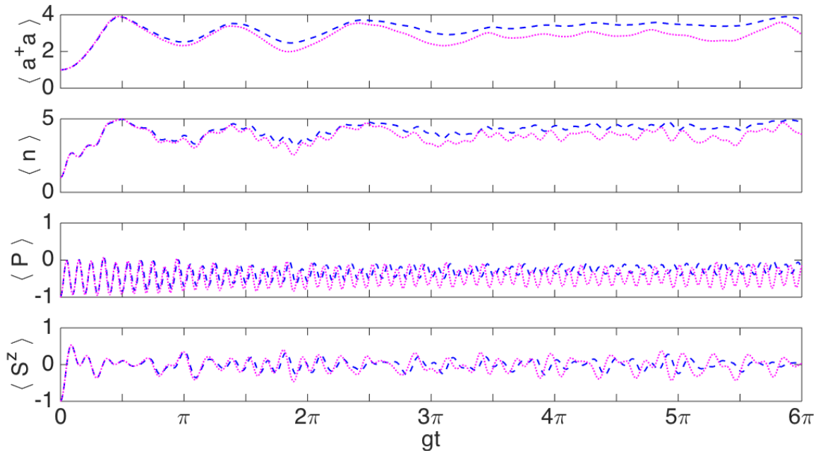
FIG. 6. Simulation of the biased Dicke model in a two trapped-ion system in the USC regime with parameters \nu = 2\pi \times 3\text{MHz} , \omega^0 = 2\pi \times 10^{14}\text{Hz} , \Omega = 2\pi \times 50\text{kHz} , \eta = 0.05 , \Gamma = \Omega\eta/100 , h = 5\Omega\eta/2 , \delta^r = -2\pi \times 100\text{Hz} and \delta^b = -2\pi \times 2.7\text{kHz} . Initial state: |1, \downarrow, \downarrow\rangle . Dotted magenta lines: biased Dicke model, dashed blue lines: ion system.
