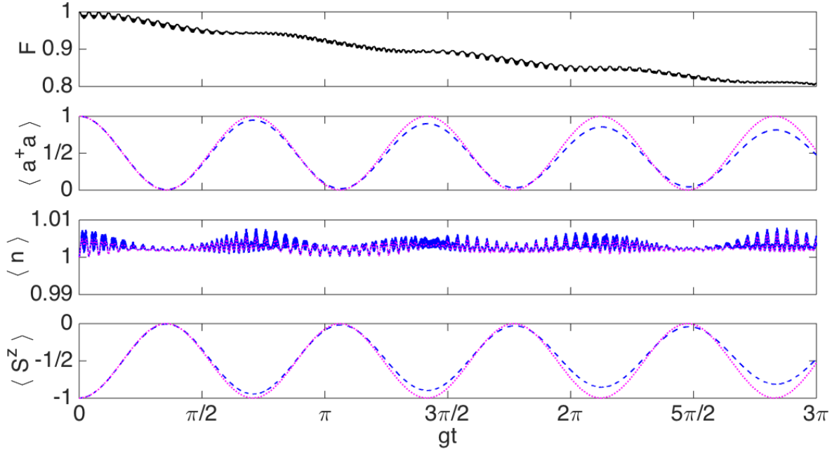
FIG. 3. Simulation of the biased Dicke model in a two trapped-ion system in the WF regime with parameters \nu = 2\pi \times 3\text{MHz} , \omega^0 = 2\pi \times 10^{14}\text{Hz} , \Omega = 2\pi \times 50\text{kHz} , \eta = 0.05 , \Gamma = \Omega\eta/100 , h = \Omega\eta/2 , \delta^r = 0 and \delta^b = -2\pi \times 125\text{kHz} . Initial state: |1, \downarrow, \downarrow\rangle . Dotted magenta lines: biased Dicke model, dashed blue lines: ion system.
