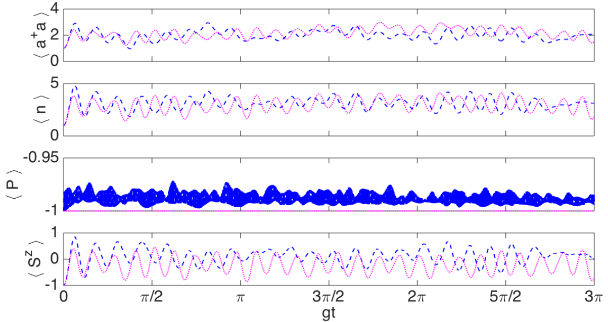
FIG. 8. Simulation of the anisotropic Dicke model in a two trapped-ion system in the USC regime with parameters \nu = 2\pi \times 3\text{MHz} , \omega^0 = 2\pi \times 10^{14}\text{Hz} , \eta = 0.05 , \Gamma = \Omega\eta/100 , \Omega^r = 2\pi \times 50\text{kHz} , s = 5 , \delta^r = -2\pi \times 100\text{Hz} and \delta^b = -2\pi \times 12.7\text{kHz} . Initial state: |1, \downarrow, \downarrow\rangle . Dotted magenta lines: anisotropic Dicke model, dashed blue lines: ion system.
