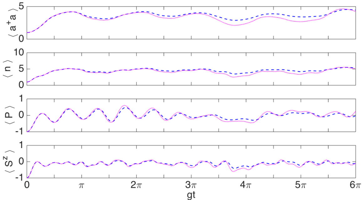
FIG. 5. Simulation of the biased Dicke model in a two trapped-ion system in the USC regime with parameters \nu = 2\pi \times 3\text{MHz} , \omega^0 = 2\pi \times 10^{14}\text{Hz} , \Omega = 2\pi \times 50\text{kHz} , \eta = 0.05 , \Gamma = \Omega\eta/100 , h = \Omega\eta/2 , \delta^r = -2\pi \times 100\text{Hz} and \delta^b = -2\pi \times 2.7\text{kHz} . Initial state: |1, \downarrow, \downarrow\rangle . Dotted magenta lines: biased Dicke model, dashed blue lines: ion system.
