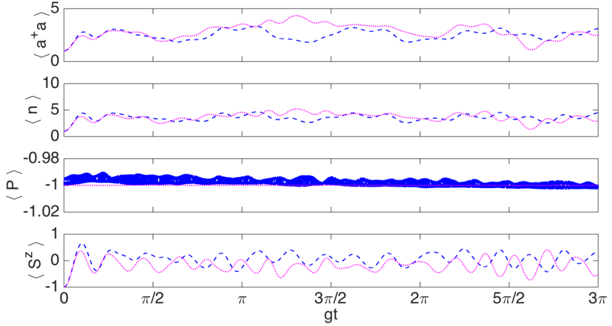
FIG. 7. Simulation of the anisotropic Dicke model in a two trapped-ion system in the USC regime with parameters \nu = 2\pi \times 3\text{MHz} , \omega^0 = 2\pi \times 10^{14}\text{Hz} , \eta = 0.05 , \Gamma = \Omega\eta/100 , \Omega^r = 2\pi \times 50\text{kHz} , s = 3 , \delta^r = -2\pi \times 100\text{Hz} and \delta^b = -2\pi \times 7.7\text{kHz} . Initial state: |1, \downarrow, \downarrow\rangle . Dotted magenta lines: anisotropic Dicke model, dashed blue lines: ion system.
