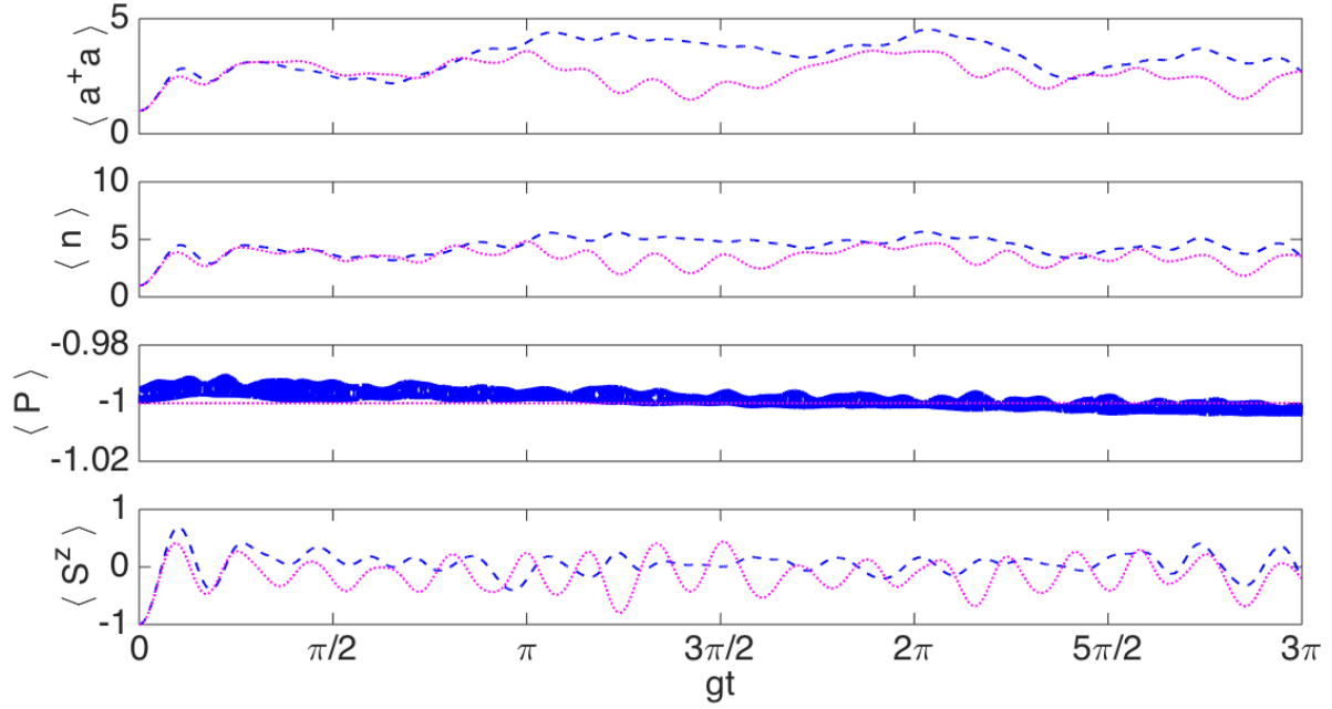
FIG. 9. Simulation of the anisotropic Dicke model in a two trapped-ion system in the DSC regime with parameters \nu = 2\pi \times 3\text{MHz} , \omega^0 = 2\pi \times 10^{14}\text{Hz} , \eta = 0.05 , \Gamma = \Omega\eta/100 , \Omega^r = 2\pi \times 50\text{kHz} , s = 3 , \delta^r = -2\pi \times 112\text{Hz} and \delta^b = -2\pi \times 7238\text{Hz} . Initial state: |1, \downarrow, \downarrow\rangle . Dotted magenta lines: anisotropic Dicke model, dashed blue lines: ion system.
