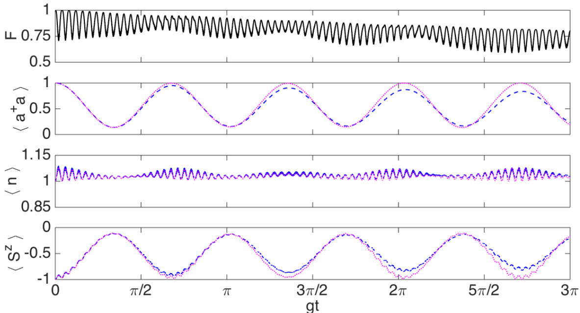
FIG. 4. Simulation of the biased Dicke model in a two trapped-ion system in the WF regime with parameters \nu = 2\pi \times 3\text{MHz} , \omega^0 = 2\pi \times 10^{14}\text{Hz} , \Omega = 2\pi \times 50\text{kHz} , \eta = 0.05 , \Gamma = \Omega\eta/100 , h = 5\Omega\eta/2 , \delta^r = 0 and \delta^b = -2\pi \times 125\text{kHz} . Initial state: |1, \downarrow, \downarrow\rangle . Dotted magenta lines: biased Dicke model, dashed blue lines: ion system.
