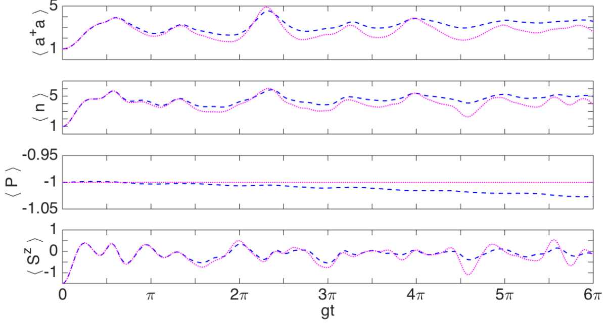
FIG. 2. Simulation of the Dicke model with three trapped ions in the USC regime with parameters \nu = 2\pi \times 3\text{MHz} , \omega^0 = 2\pi \times 10^{14}\text{Hz} , \Omega = 2\pi \times 50\text{kHz} , \eta = 0.05 , \Gamma = \Omega\eta/100 , \delta^r = -2\pi \times 100\text{Hz} and \delta^b = -2\pi \times 2.7\text{kHz} . Initial state: |1, \downarrow, \downarrow, \downarrow\rangle . Dotted magenta lines: Dicke model, dashed blue lines: ion system.
