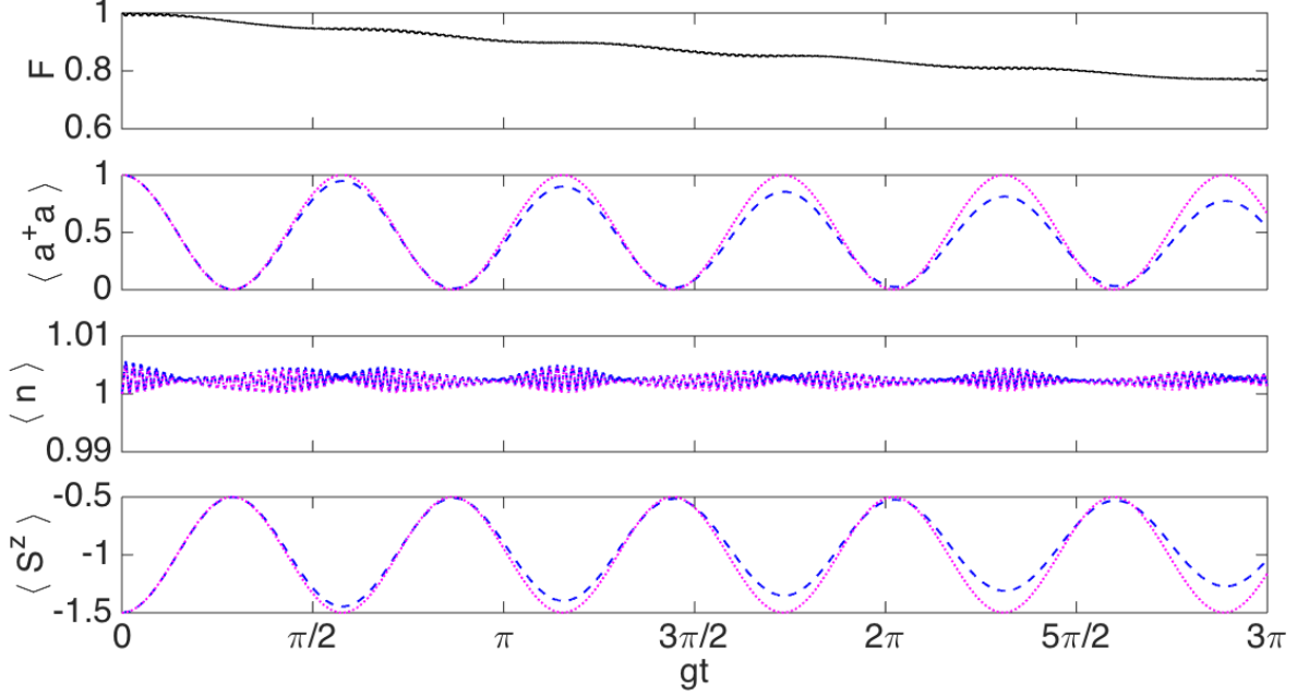
FIG. 1. Simulation of the Dicke model with three trapped ions in the WF regime with parameters \nu = 2\pi \times 3\text{MHz} , \omega^0 = 2\pi \times 10^{14}\text{Hz} , \Omega = 2\pi \times 50\text{kHz} , \eta = 0.05 , \Gamma = \Omega\eta/100 , \delta^r = 0 and \delta^b = -2\pi \times 125\text{kHz} . Initial state: |1, \downarrow, \downarrow, \downarrow\rangle . Dotted magenta lines: Dicke model, dashed blue lines: ion system.
