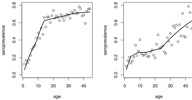
FIG. 2. Seroprevalence of Parvovirus B19 (left panel) and Cytomegalovirus (right panel) infections with age (years). The lines show the fitted values obtained from the model with shared frailty U(t) \propto U^{h(t)} with gamma U and exponentially declining h(t) .
