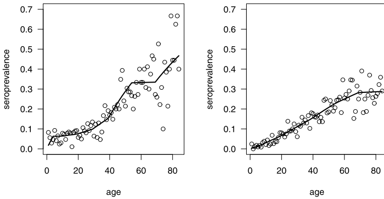
FIG. 4. Seroprevalence of Helicobacter pylori (left panel) and Toxoplasma (right panel) infections with age (years). The lines show the fitted values obtained from the model with shared frailty U(t) \propto U^{h(t)}V with gamma U and V and exponentially declining h(t) .
