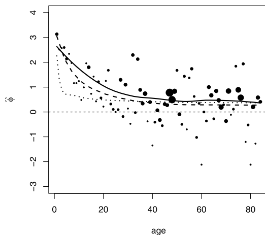
FIG. 5. Association between Helicobacter pylori and Toxoplasma by age (years). The dots represent the empirical values of the association parameter \hat{\phi} (with area inversely proportional to the empirical variance of \hat{\phi} ). The full line is a LOESS curve. The curved dashed line shows the fitted values obtained from the model with shared frailty U(t) \propto U^{h(t)}V with gamma U and V and exponentially declining h(t) . The curved dotted line shows the fitted values obtained from the model with time-invariant generalized gamma frailty U . The horizontal dashed line represents no association.
