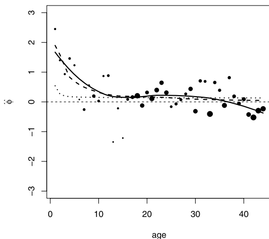
FIG. 3. Association between Parvovirus B19 and Cytomegalovirus by age (years). The dots represent the empirical values of the association parameter \hat{\phi} (with area inversely proportional to the empirical variance of \hat{\phi} ). The full line is a LOESS curve. The curved dashed line shows the fitted values obtained from the model with shared frailty U(t) \propto U^{h(t)} with gamma U and exponentially declining h(t) . The curved dotted line shows the fitted values obtained from the model with time-invariant generalized gamma frailty U . The horizontal dashed line represents no association.
