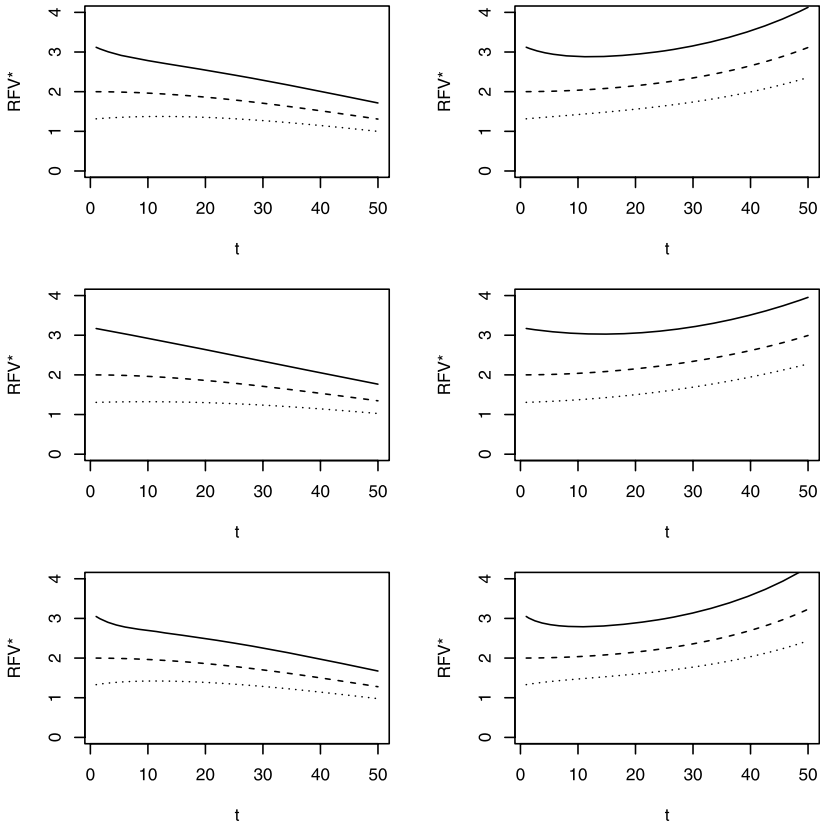
FIG. 1. Relative frailty variance function RFV^*(t) for time-varying generalized gamma frailty U^{h(t)} with E(U) = 1 and h(t) = \exp(-\rho t^2) . Parameter values are k = 0.5 and, top to bottom in each panel, \beta = 0.8, 1, 1.25 . Left panels: h(t) decreasing ( \rho = 0.0001 ). Right panels: h(t) increasing ( \rho = -0.0001 ). Top panels: hazard constant, \lambda(t) = e^{-3.34} . Middle panels: hazard increasing, \lambda(t) = \exp(-4.5 + t/25) . Bottom panels: hazard decreasing, \lambda(t) = \exp(-2.5 - t/25) .
