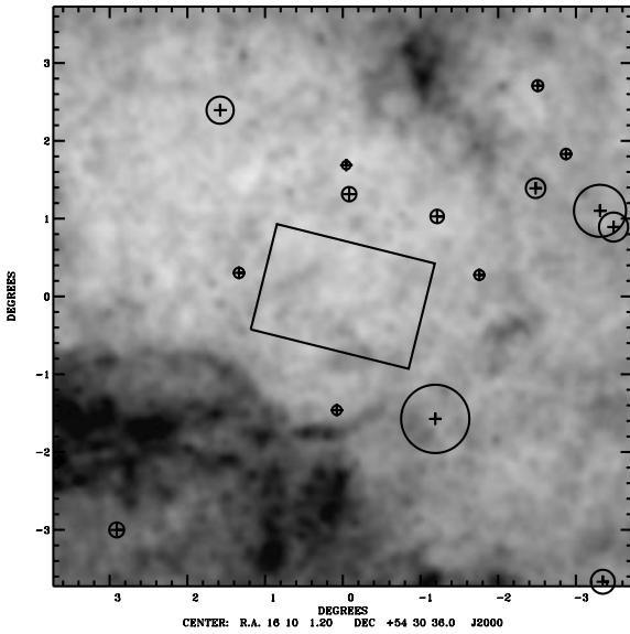
Figure 8. The location of the N1 ELAIS survey field overlaid on the COBE normalized IRAS maps of Schlegel et al. (1998). IRAS sources with 12\text{-}\mu\text{m} fluxes brighter than 0.6\text{ Jy} are overlaid with radius proportional to flux for S_{60} < 10\text{ Jy} . The minimum 100\text{-}\mu\text{m} intensity shown is 0\text{ MJy sr}^{-1} (white) and the maximum is 1.5\text{ MJy sr}^{-1} (black).
