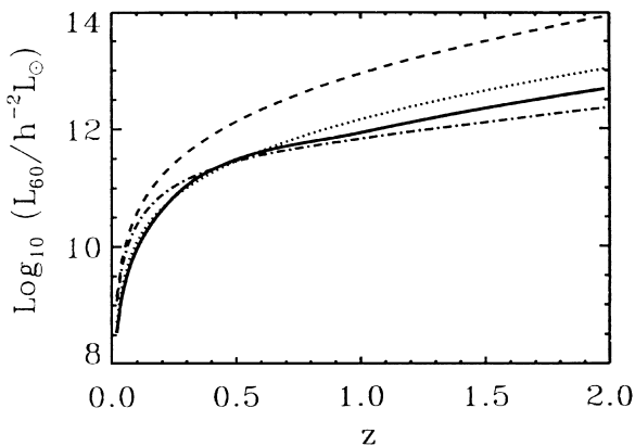
Figure 4. The minimum rest-frame 60- \mu m luminosity for a source with a starburst spectrum detectable in the ELAIS survey at S_{15} > 3 mJy (solid line), S_{90} > 100 mJy (dotted line), S_{175} > 75 mJy (dot-dashed line) and in the IRAS survey S_{60} > 250 mJy (dashed line).
