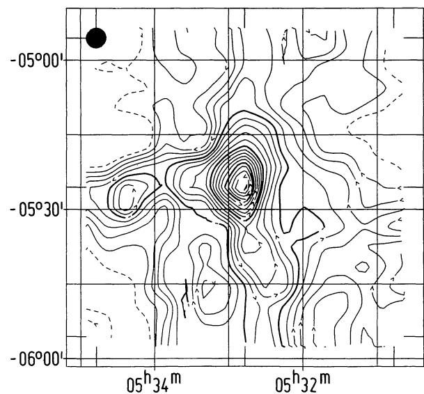
Fig. 1. CO emission observed around the Orion Nebula in a 2.6 \text{ km s}^{-1} bandwidth centred on v_{\text{lsr}} = 9 \text{ km s}^{-1} . The contour interval is 2.8 K, the zero contour is dashed and negative contours have been omitted. The smoothed beam size of 4' is shown by the circle in the north-east corner
