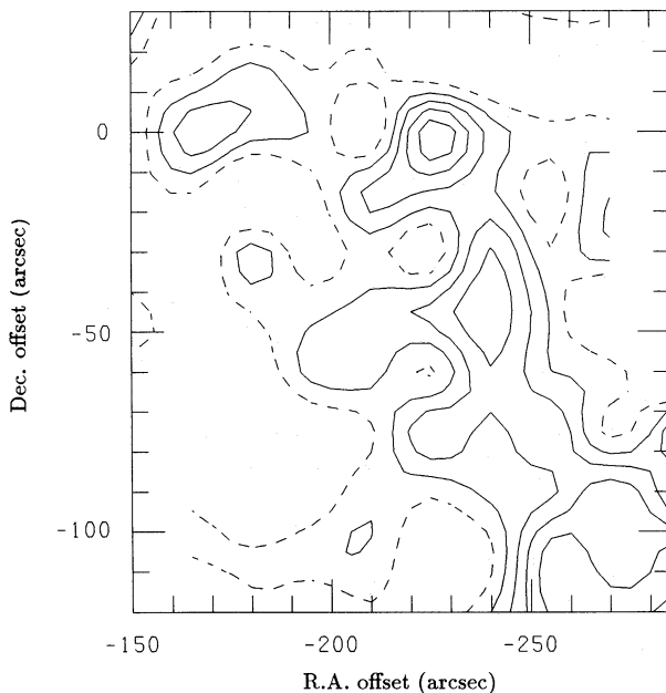
Fig. 8. The distribution of red-shifted ( 7\text{--}10\text{ km s}^{-1} ) ^{12}\text{CO } J=3-2 emission in the vicinity of HH 102. Details of the map are as for Fig. 1. Contours of integrated intensity have interval 1\text{ K km s}^{-1} , with lowest contour 6\text{ K km s}^{-1}
