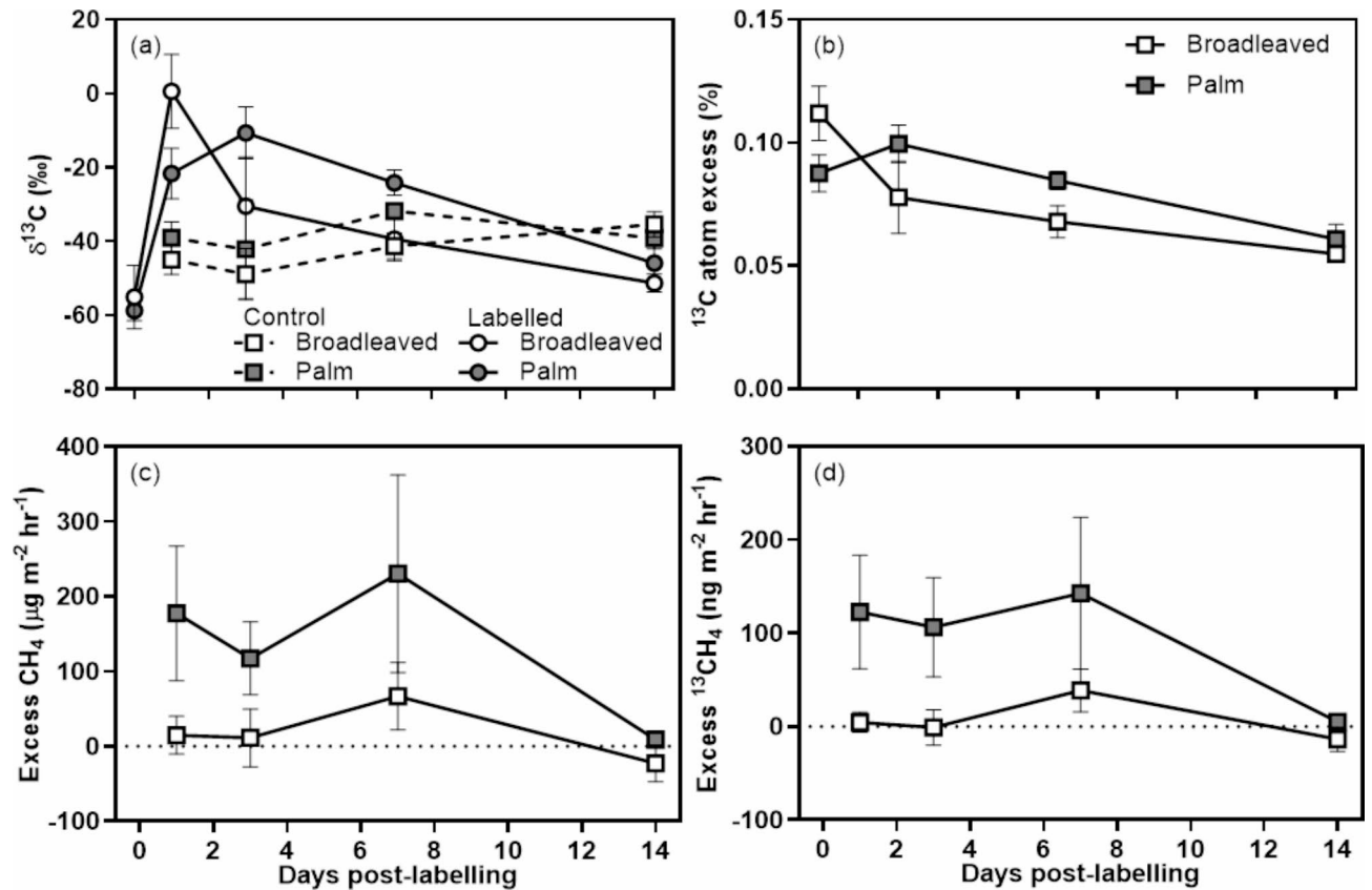
Fig. 3. (a) \delta^{13}\text{C} of emitted \text{CH}_4 , (b) Atom excess ^{13}\text{CH}_4 , (c) excess \text{CH}_4 fluxes, (d) excess ^{13}\text{CH}_4 for broadleaved evergreen and palm plant types. Means \pm 1 SE (broadleaved n = 5 , palm n = 4 ).
