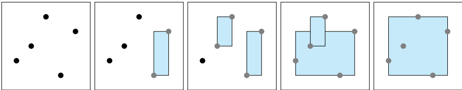
FIGURE 1. A 3-wide merge sequence of 23514. Black points are also degenerate rectangles.
