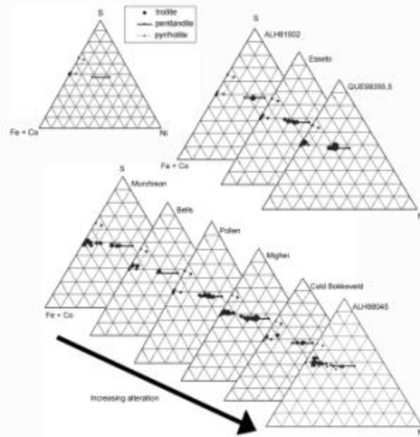
Fig. 1. Triangular diagrams showing the compositional range of Fe-Ni sulphides in CM1 and CM2 carbonaceous chondrites. Bottom row of diagrams shows increasing alteration, according to [8]; top row of diagrams shows CM2s not included in the study by [8].
