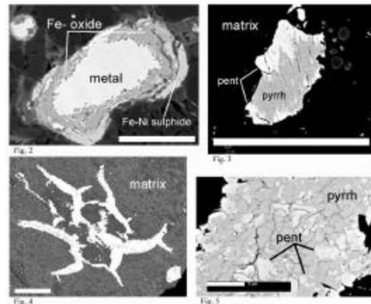
Fig. 2. Metal grain with Fe-oxide and Fe-Ni sulphide rims in Mighei. Scale bar is 30\mu\text{m} . Fig. 3. Intergrown pyrrhotite and pentlandite in Essebi. Fig. 4. BSE image of intergrown pyrrhotite and pentlandite (white) in matrix (grey) in ALH88045. Scale bar is 200\mu\text{m} . Fig. 5 High-contrast image of intergrown pyrrhotite and pentlandite in ALH88045. Scale bar is 5\mu\text{m} .
