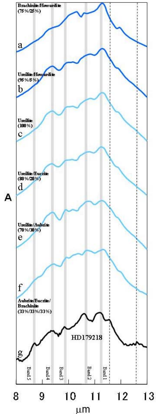
Fig.1a-g. Spectra of differentiated meteorites (a)-(f) (in brackets percentages of specific meteorites in calculated mixtures of different spectra). (a) and (b) are mixtures calculated using a least square routine. For comparison, the astronomical spectrum of HD179218 (g). When single spectra or binary mixtures are used, spectra dominated by Ureilites show a good similarity to this astronomical spectra (b)-(e). A mixture of three different types of achondrites (f) also gives a good result.
