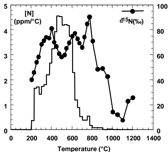
Figure 2: Nitrogen in Tagish Lake
