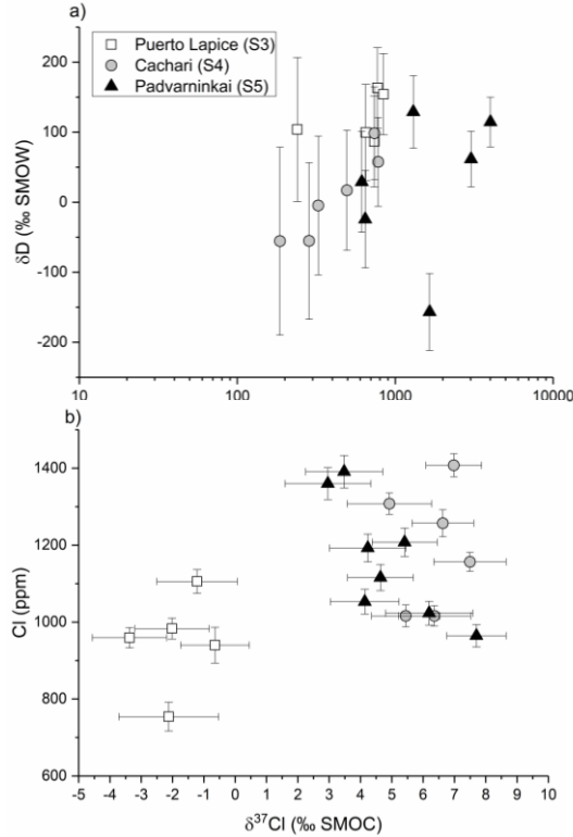
Figure 1: a) Plot of \delta D values versus H_2O content of analyzed samples. b) \delta^{37}Cl values versus Cl content.
