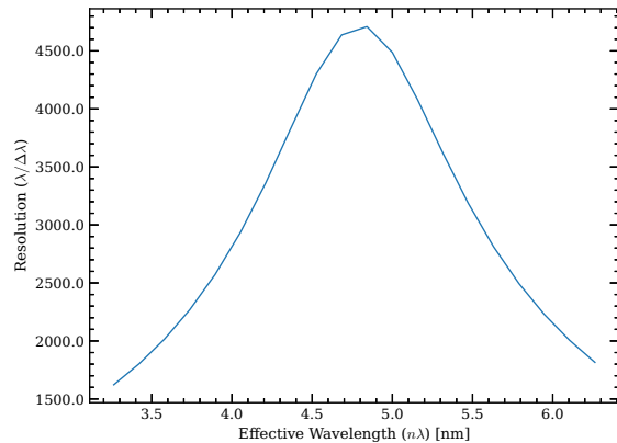
Figure 6. Theoretical resolution response of the OGRE spectrograph around the effective blaze wavelength ( n\lambda_b = 4.76 nm). The resolution of the spectrograph peaks around the blaze wavelength, where spectral detectors were placed to maximize observed resolution, and falls off rapidly outside the wavelength of interest due to path length differences.
