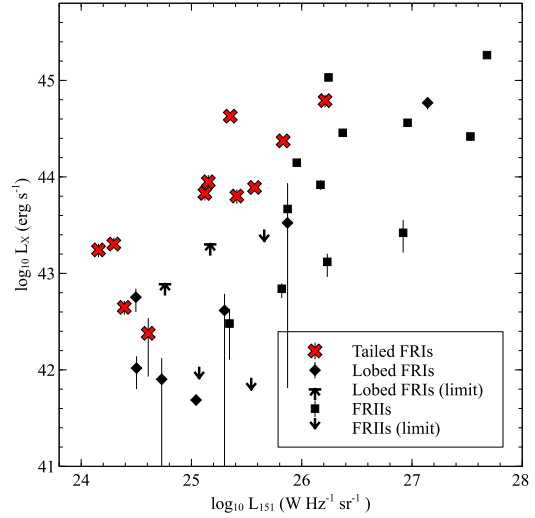
Figure 3. The X-ray environment – radio luminosity relation for LERGs, from Ineson et al. (2015), broken down by radio morphology. A small number of upper limits on the X-ray environmental luminosity are present, as indicated in the legend.
