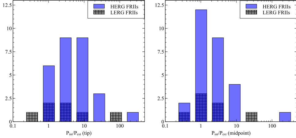
Figure 6. Pressure ratio comparison for FRIIs, broken down by accretion mode. Low-excitation FRII radio galaxies (LERGs) are indicated by hatched black regions, while high-excitation FRIIs (HERGs) are shown in blue. Pressures are the inverse-Compton derived pressures from I17, with pressure ratio limits omitted.
