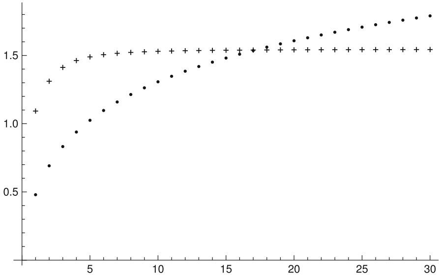
Fig. 1 Values of \log(\lambda) (dots) and m(q) (crosses) for 1 \leq m \leq 30
