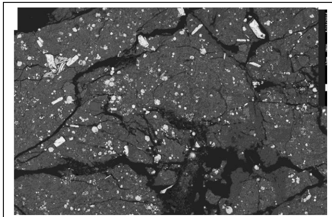
Fig. 1. BSE Image of Carancas clast. View measures 0.5 mm across. Magnetite and sulfides are white, most of the remainder is phyllosilicates and carbonates.
