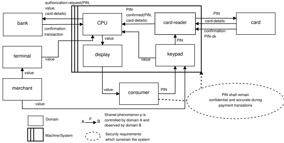
Figure 12: System context of the PED system and its security requirements
