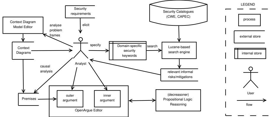
Figure 5: An overview flowchart of the OpenRISA tool support
