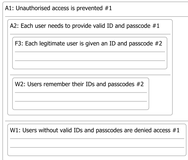
Figure 10: A nested argument
