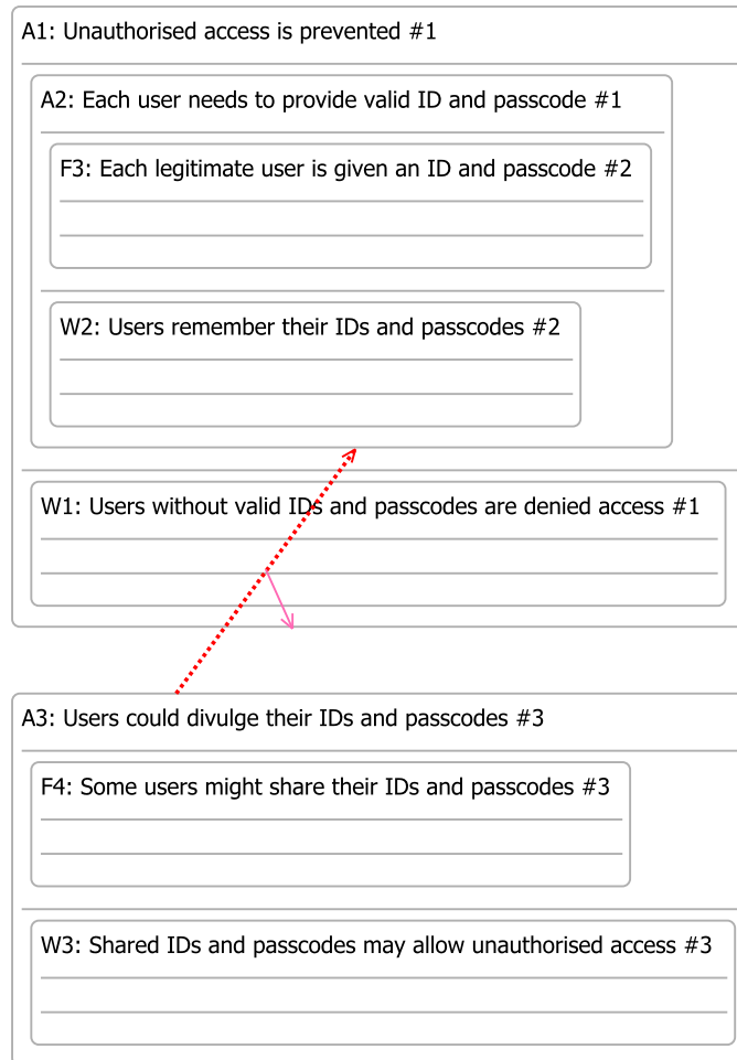
Figure 11: An argument and its rebuttal
