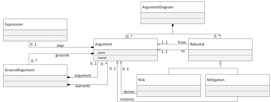
Figure 3: The metamodel of argument diagrams, the detailed structure of boolean expressions is omitted here.
