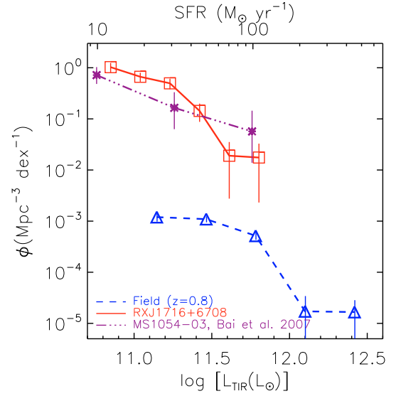
Fig. 3. Total infrared LFs of cluster RXJ1716.4+6708 at z = 0.81 in the solid line, and those of the AKARI NEP-deep field in the dashed line. Overplotted are the LFs of MS1054 from Bai et al. (2007).
