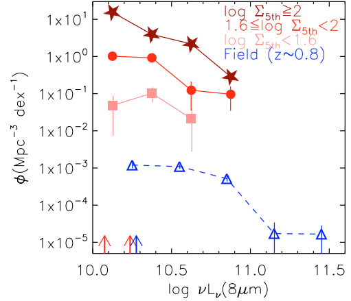
Fig. 2. Restframe 8 \mu\text{m} LFs of cluster RXJ1716.4+6708 at z = 0.81 , divided according to the local galaxy density ( \Sigma_{5\text{th}} ). The stars, circles, and squares indicate galaxies with \log \Sigma_{5\text{th}} \geq 2 , 1.6 \leq \log \Sigma_{5\text{th}} < 2 , and \log \Sigma_{5\text{th}} < 1.6 , respectively.
