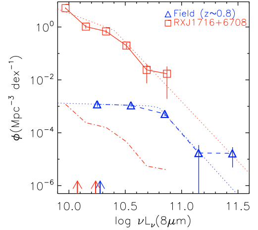
Fig. 1. Restframe 8\ \mu\text{m} LFs of cluster RXJ1716.4+6708 at z = 0.81 in the squares, and those of the AKARI NEP-deep field in the triangles. For RXJ1716.4+6708, only photometric and spectroscopic cluster member galaxies are used. For the NEP-deep field, galaxies with photo- z /spec z in the range of 0.65 < z < 0.9 are used. The dot-dashed lines are 8\ \mu\text{m} LFs of RXJ1716.4+6708, but scaled down for easier comparison. The thin dotted lines are the best-fit double power laws. Vertical arrows show the 5\sigma flux limits of deep/shallow regions of the cluster (red) and the NEP-deep field (blue) in terms of L_{8\ \mu\text{m}} at z = 0.81 .
