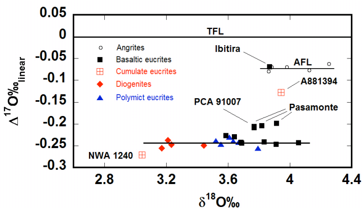
Fig. 1. Oxygen isotope variation diagram for the 22 achondrites analyzed in this study and five angrites from [2]. TFL = terrestrial fractionation line, AFL = angrite fractionation line. The line drawn through the HED data excludes outliers and is indistinguishable from that of [2].
