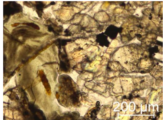
Figure 2: polarizing optical microscope image of a thin polished section of the martian meteorite NWA 4222 (sample MSP 5040). The large dark-brown-green area is glass; transmitted light, plane polars.
