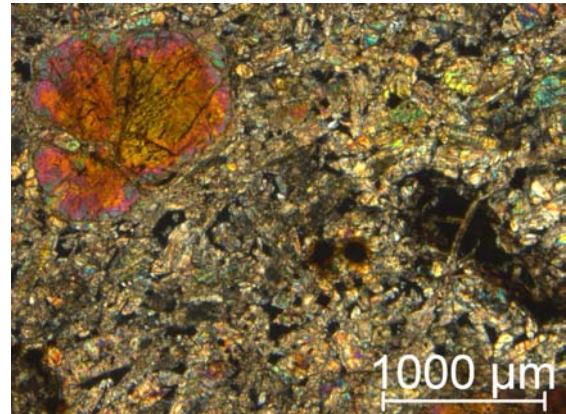
Figure 1: polarizing optical microscope image of a thin section of the martian meteorite NWA 4222 (sample MSP 5040). The rounded orange-pink grain is olivine, elongated yellow crystals are pyroxene; transmitted light, crossed polars.
