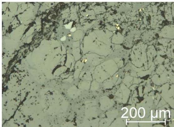
Figure 4: polarizing optical microscope image of a thin polished section of the martian meteorite NWA 4222 (sample MSP 5040). Tiny yellow grains are pyrrhotite; pale grey grains are ilmenite; reflected light, plane polars.
