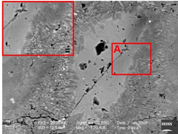
Figure 3: SEM-BSE image of the same area of figure 2; the inner pale grey area is a pigeonitic glass. This area is surrounded by glass fringes; top left: blow up of area A showing the Mg-enriched glass (dark grey) and the Fe-enriched one (white).
