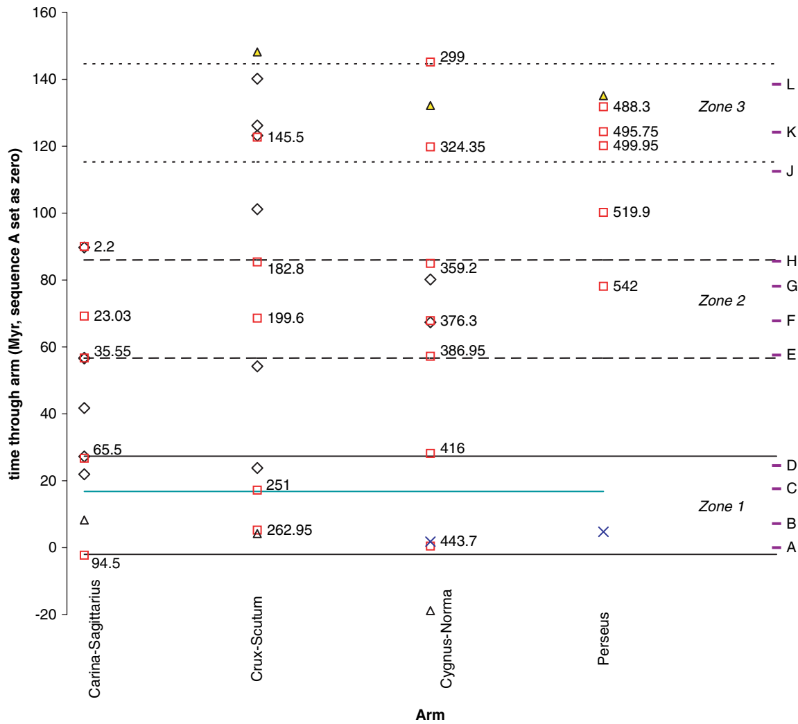
Fig. 2. Signature of events through the arms. Zones of high extinction activity are detailed in Table 2. The positions of the sequences A–L are indicated on the right-hand side. Symbols: ◇, impacts with craters \geq 40 km diameter; □, geological period/high extinction midpoint; △, yellow, start of superchron and clear, end of superchron; and ×, large early impacts. The blue line in Zone 1 indicates the position of the spiral arm midpoints (Figure 1). Values for extinction/geological period points are absolute ages in contrast to the vertical axis, which shows time through the arm from sequence A. The two large early impacts occurred at 1850 and 2023 mya (equivalent to arms 11 and 12, i.e. Cygnus and Perseus), placing them between sequences A and B.
